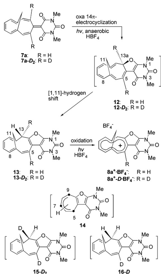
Scheme 3. Reaction pathway for the photoinduced oxidative cyclization.
