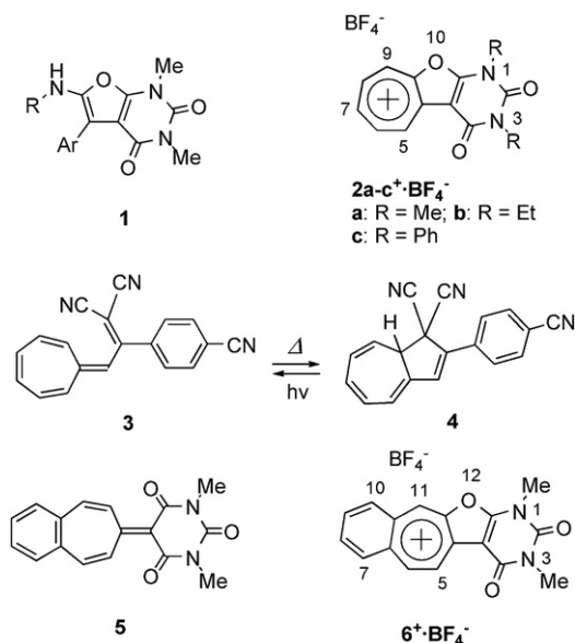
Figure 1. Furo[2,3- d ]pyrimidine derivatives and heptafulvenes.
