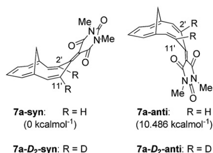
Figure 2. Two possible conformations of 7a and 7a-D 2 .
