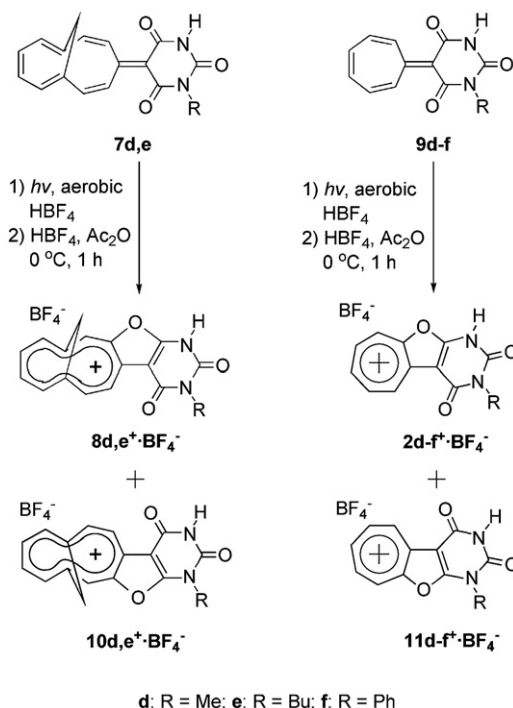
Scheme 2. Photoinduced oxidative cyclization of mono-substituted compounds 7d,e and 9d–f .
