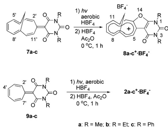
Scheme 1. Photoinduced oxidative cyclization of disubstituted compounds 7a–c and 9a–c .
